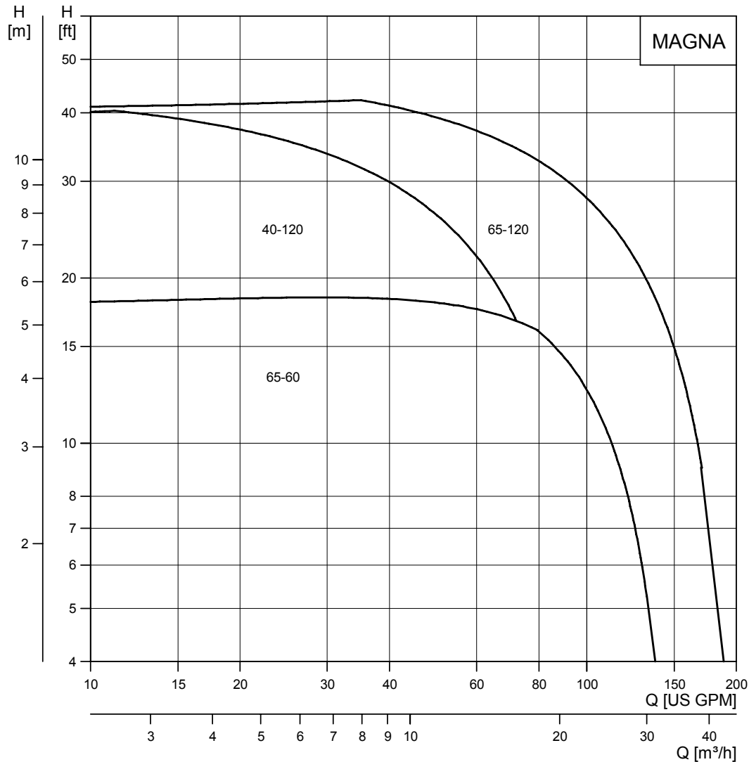
Fig. 2 Performance range
