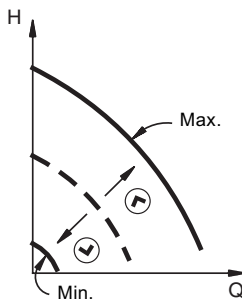
Fig. 8 Constant-curve duty
