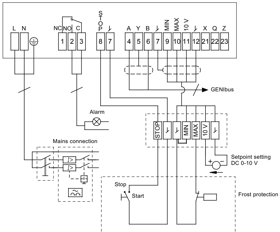
Fig. 22 Example of MAGNA pump with GENI module
