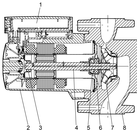
Fig. 16 MAGNA 40-120, 65-60 and 65-120
