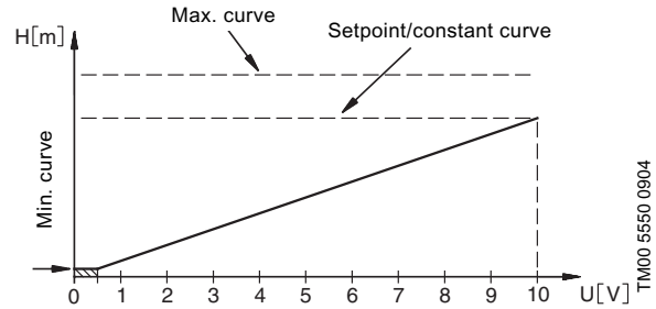
Fig. 13 Example of 0-10 V control
