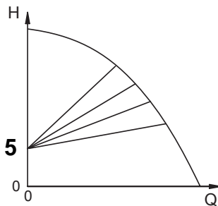
Fig. 4 AUTOADAPT control
