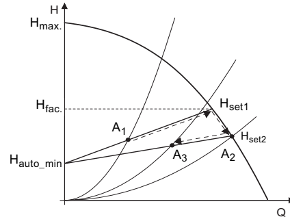
Fig. 5 AUTOADAPT
