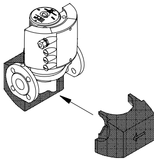
Fig. 23 Fitting the insulating shells to a MAGNA pump
