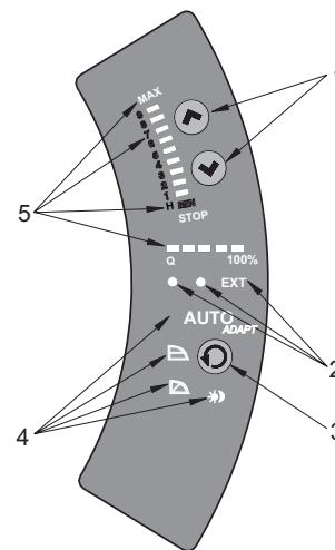
Fig. 11 MAGNA control panel
