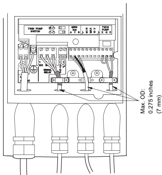
Fig. 19 Two pumps in parallel, master
