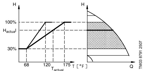
Fig. 10 Temperature influence
