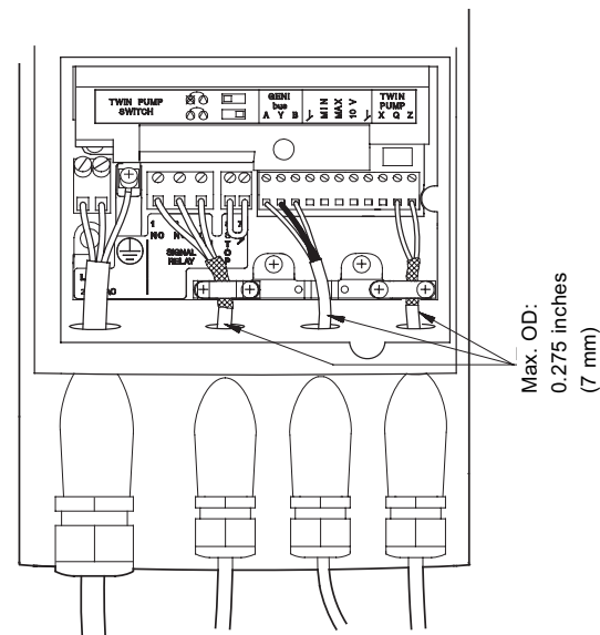
Fig. 20 Two pumps in parallel, slave
