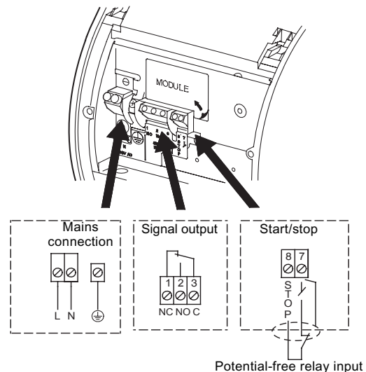
Fig. 18 MAGNA 40-120, 65-120, 65-60, mains connection
