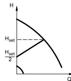
Fig. 6 Proportional-pressure control
