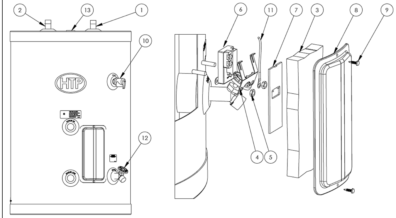
Figure 8 – Parts Blowout
