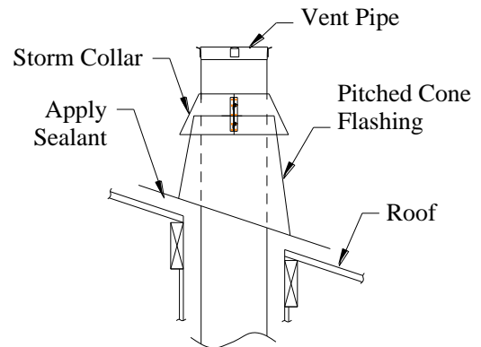
Fig 18. (Pitched Cone Flashing)
