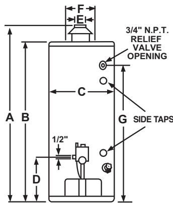
G50-65, G60-50, G65-65, G75-75 & G100-65 SIDE TAPS ON 48, 63, 75 & 98 GAL. MODELS ONLY
