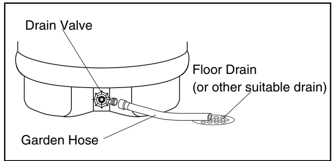
Figure 12 - Draining the Tank
