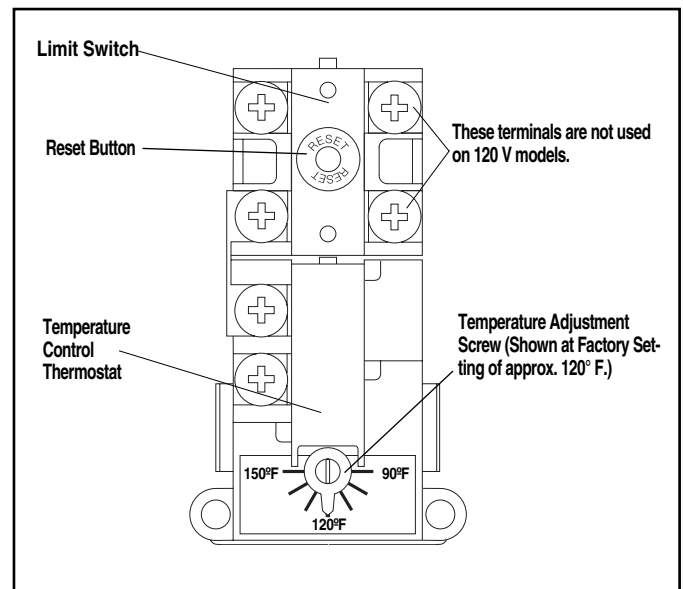
Figure 11 — Thermostat & High Limit Switch
