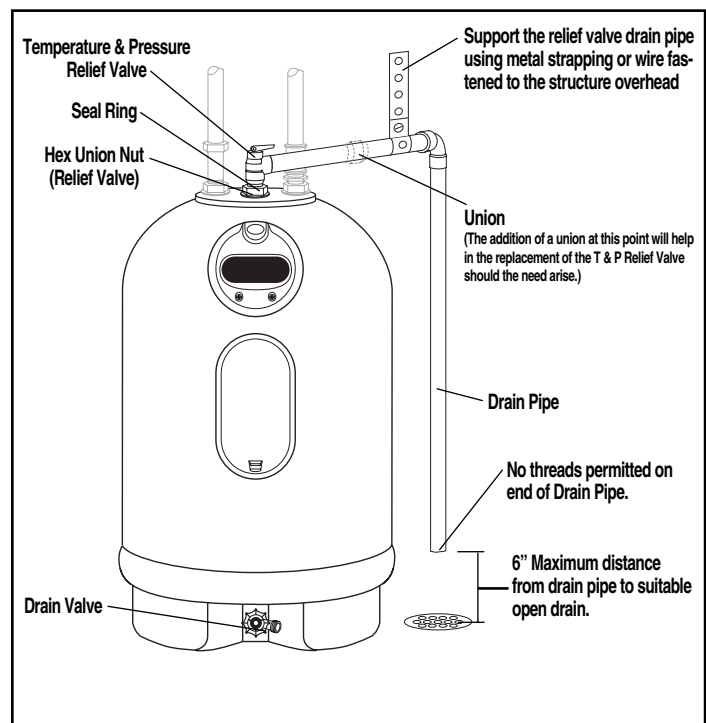
Figure 3 — Typical method of supporting relief valve drain pipe.
