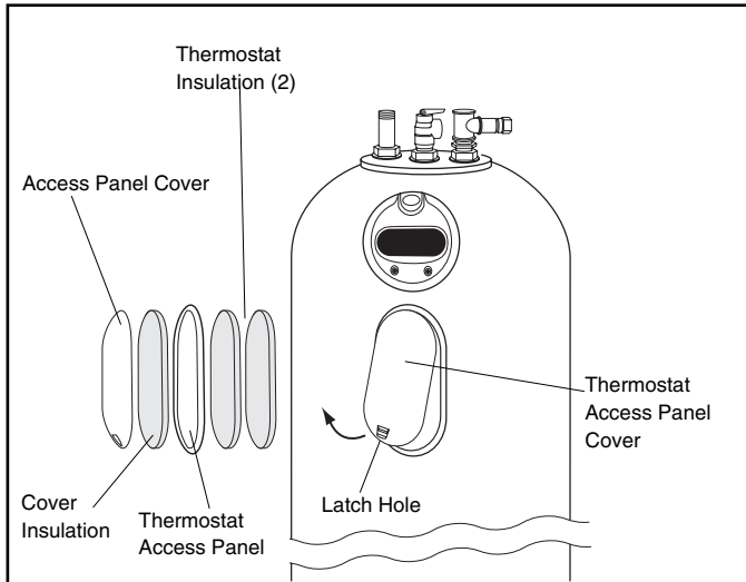
Figure 9 — Removing Thermostat Access panel.
