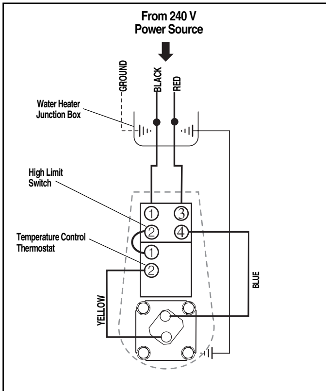
Figure 6 — Complete Wiring Schematic Diagram —240 Volt Units
