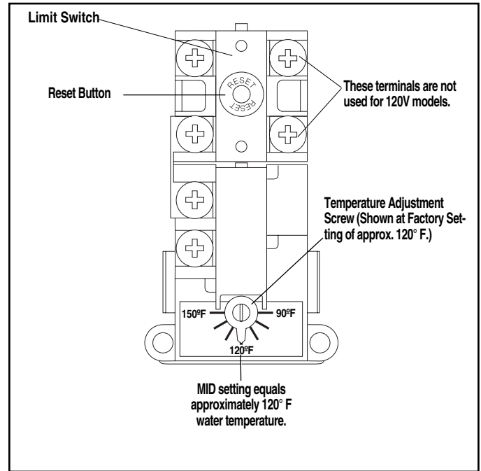
Figure 10 — Thermostat temperature adjustment.
