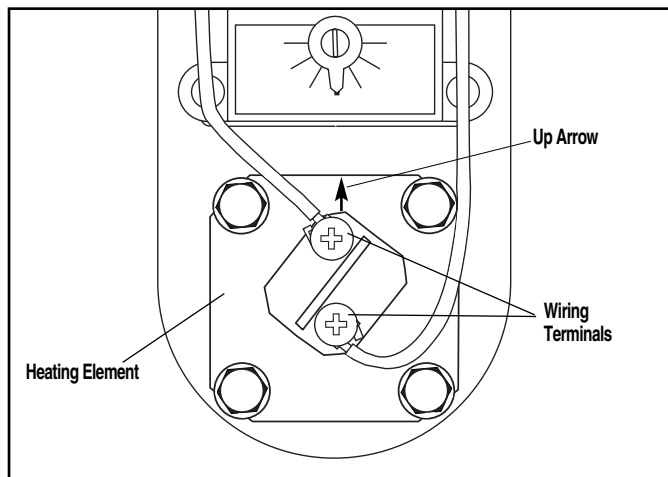
Figure 15. — Typical Element Wiring
