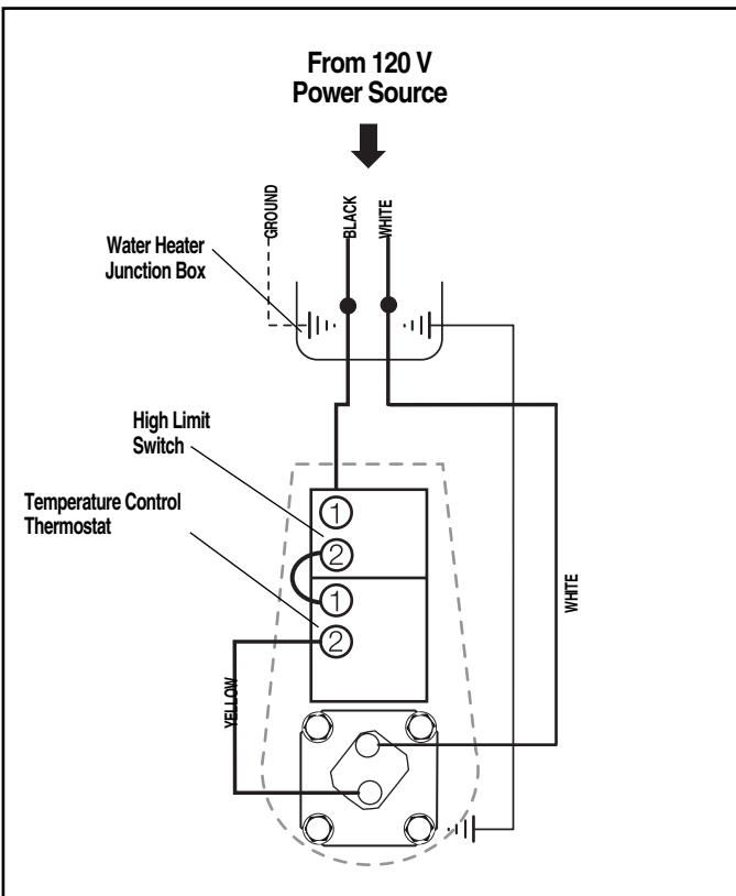
Figure 7 — Complete Wiring Schematic Diagram — 120 Volt Units
