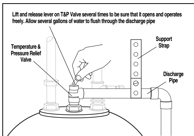
Figure 13 — Manually Operating the Temperature and Pressure Relief Valve
